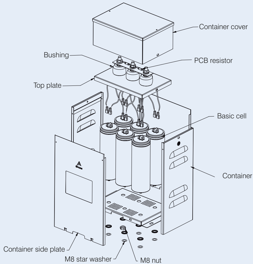
SquareCap : Exploded view
