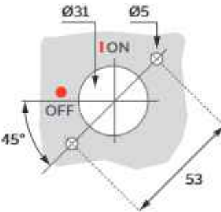
Door drilling for OH_handles:
