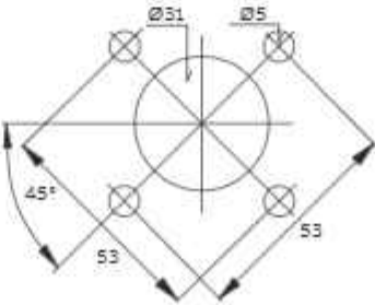
Door drilling for OHB_handles:
