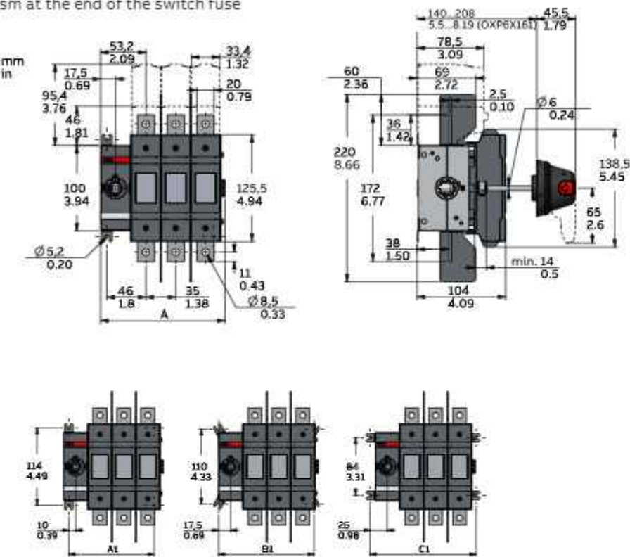
OS100GJ_ Mechanism at the end of the switch fuse
