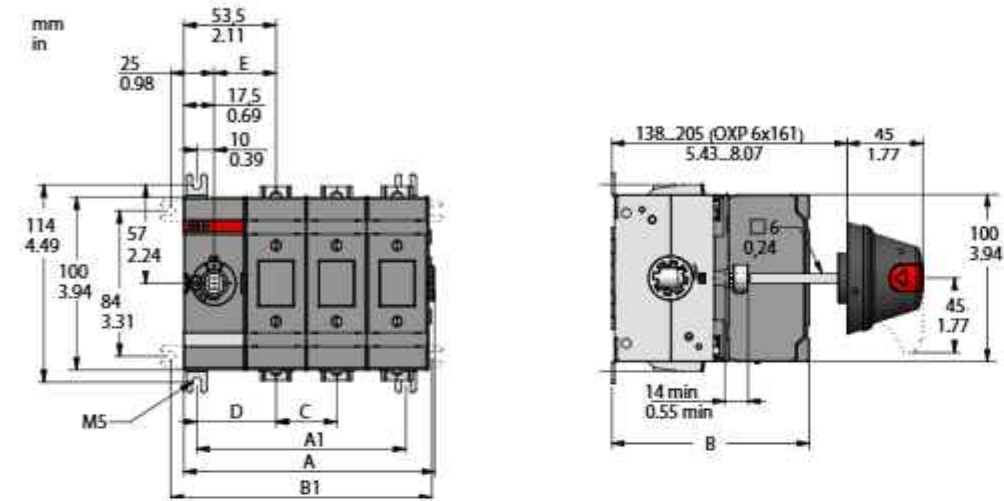
OS60GJ_ Mechanism at the end of the switch fuse
