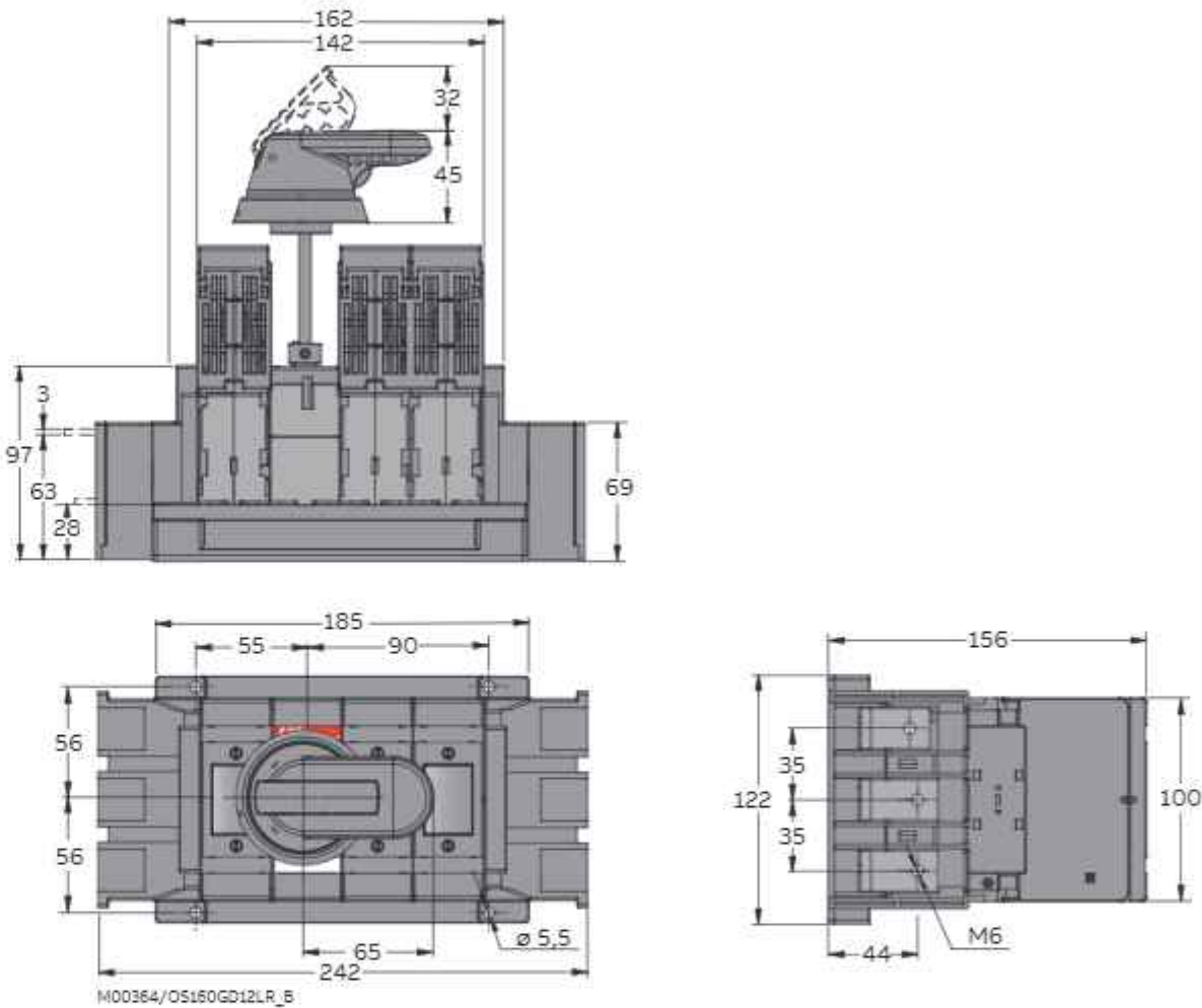
OS125G...160GD12LR (LR)
