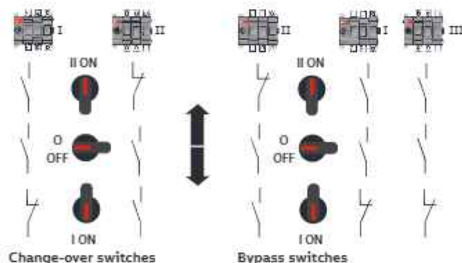
Change-over switches
