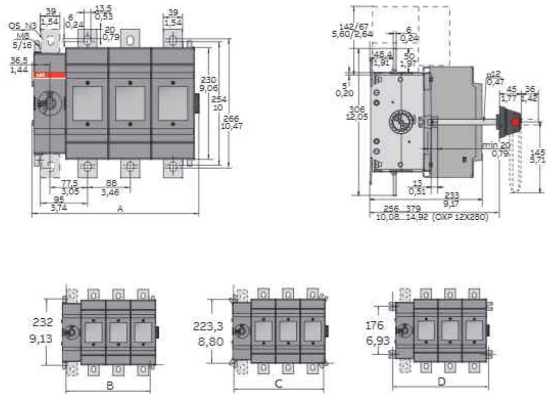
OS600J and OS800L Mechanism at the end of the switch fuse
