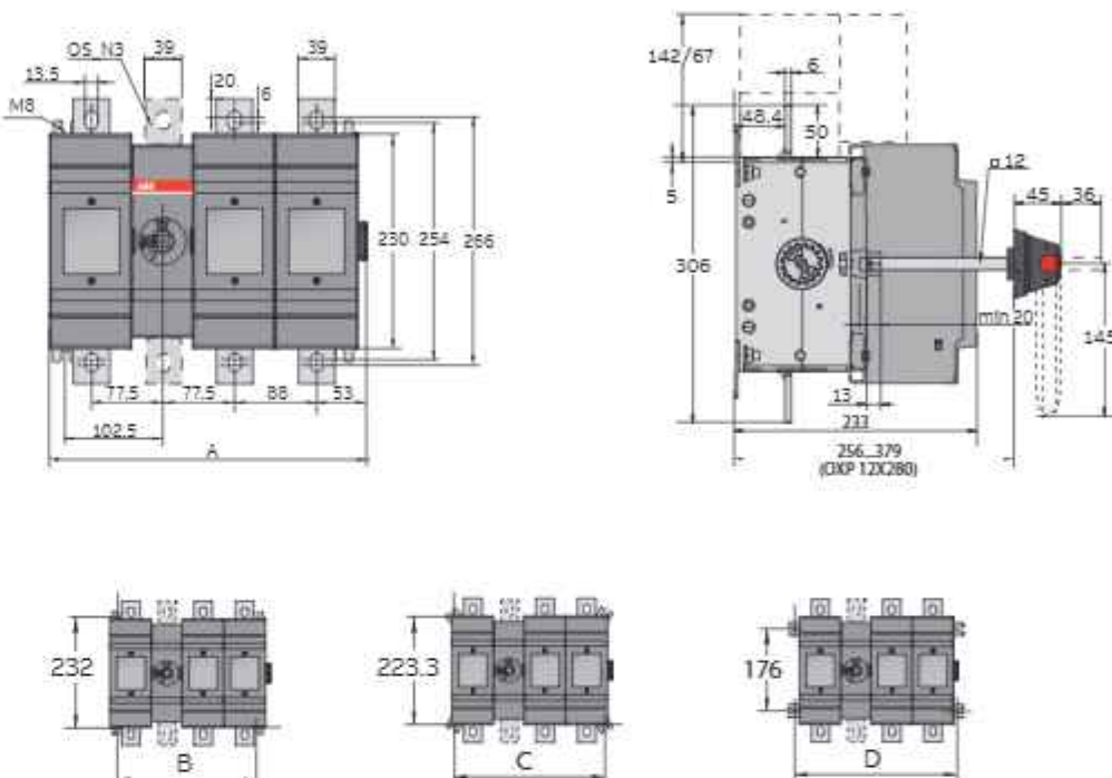
OS 630_P and OS 800_P Mechanism between the poles
