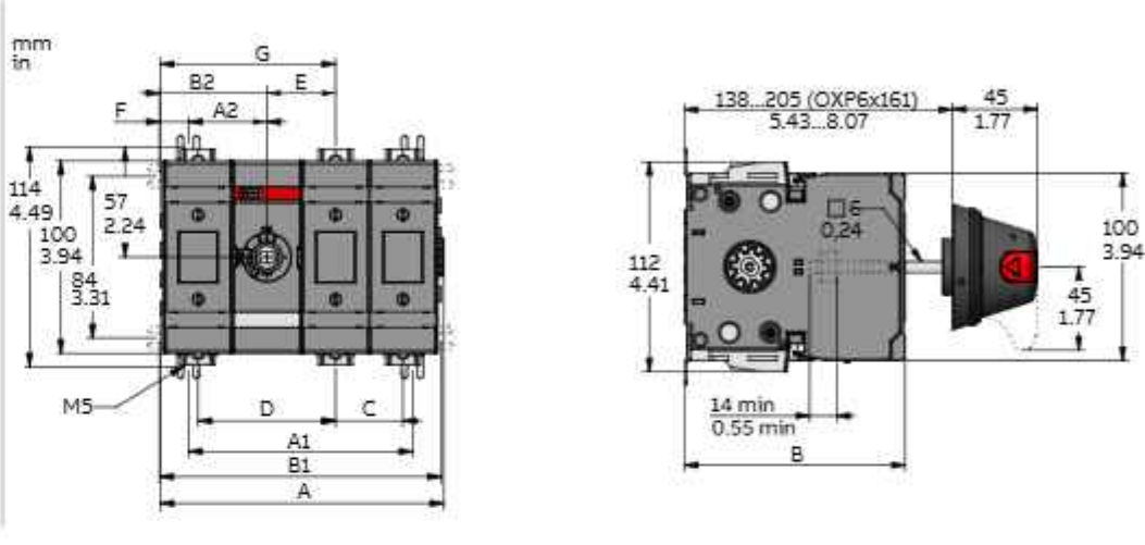
OS60GJ_ Mechanism between the poles
