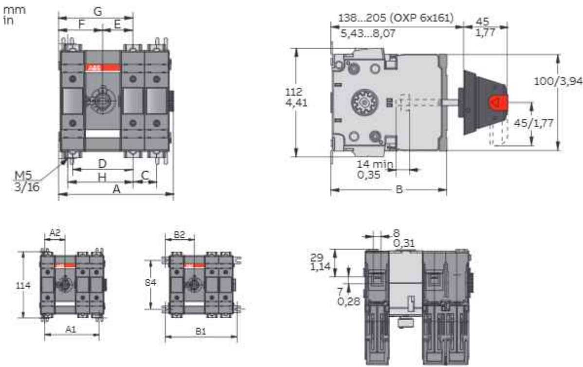
OS32...63G_P Mechanism between the poles
