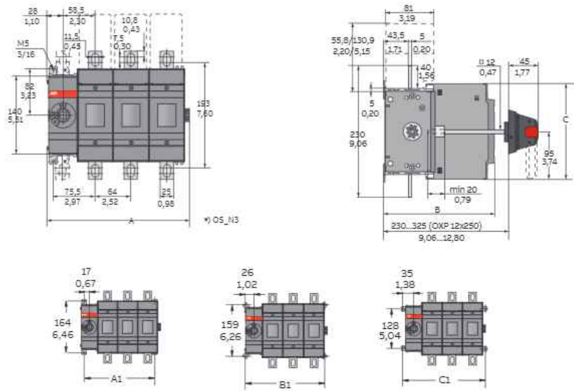
OS400J Mechanism at the end of the switch fuse
