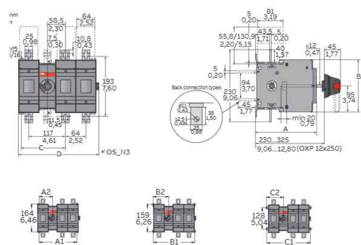
OS315_12/22_ and OS400_12/22 (BB)
